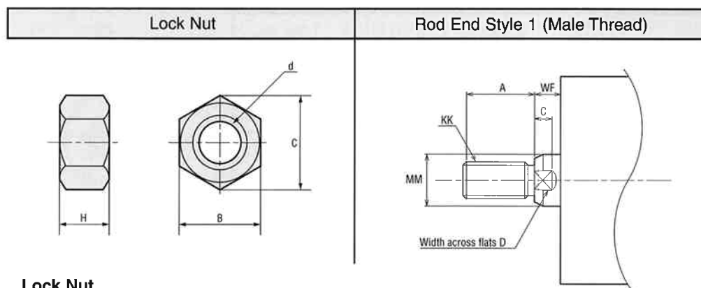
Lock Nut
